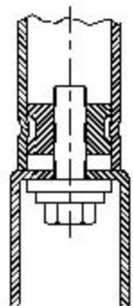
Enlarged Section F-F
