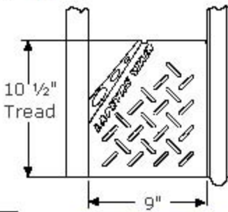
Enlarged Section E-E
